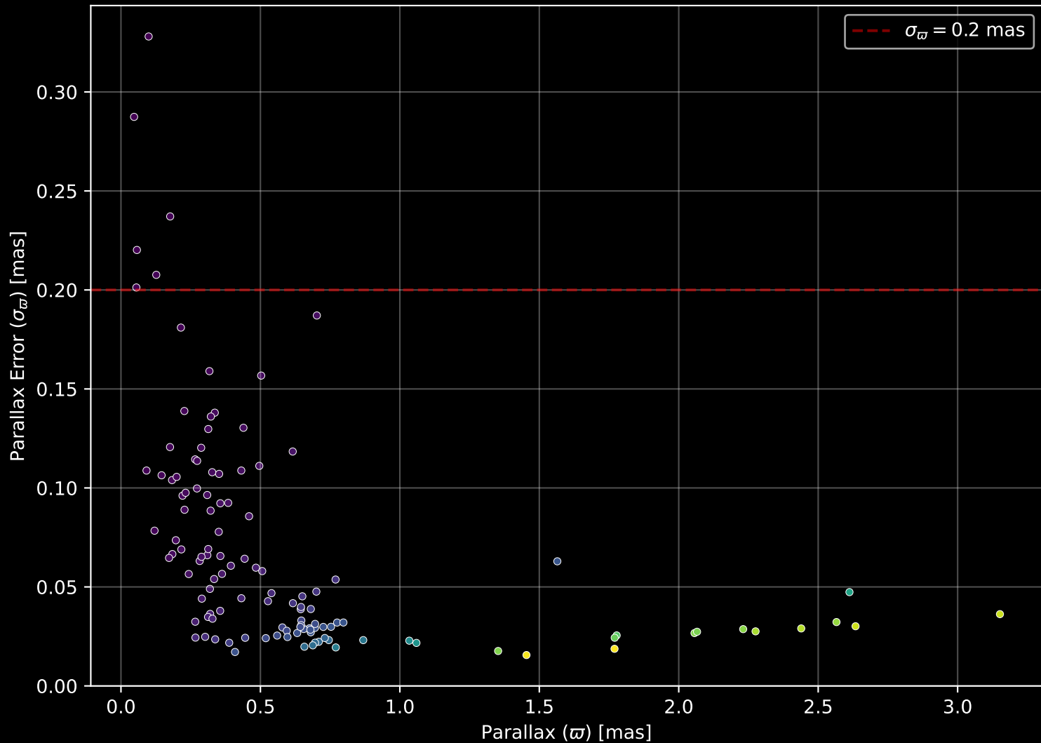
APOGEE DR17 Field: [014+00] Parallax Quality (n= 122)
