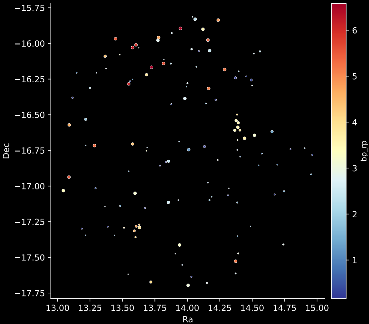
APOGEE DR17 Field: [014+00] Stars: 122
