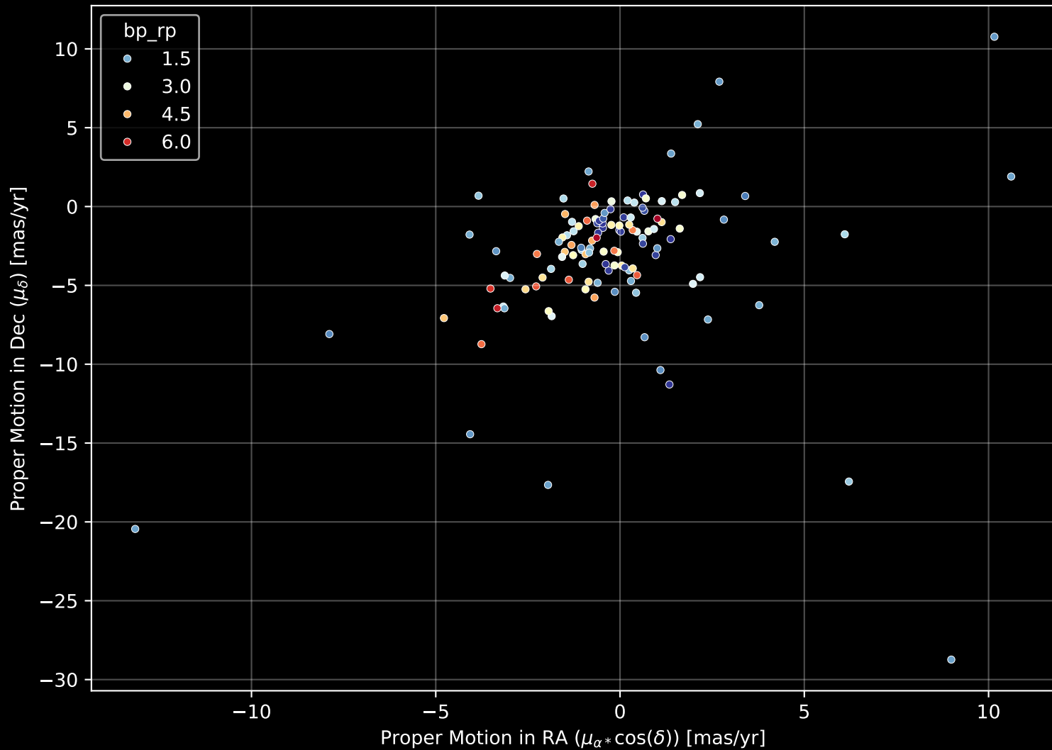
APOGEE DR17 Field: [014+00] Proper Motion Diagram (n= 122)
