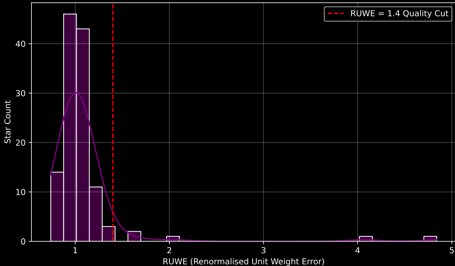
GAPOGEE DR17 Field [014+00] RUWE Distribution (n= 122)
