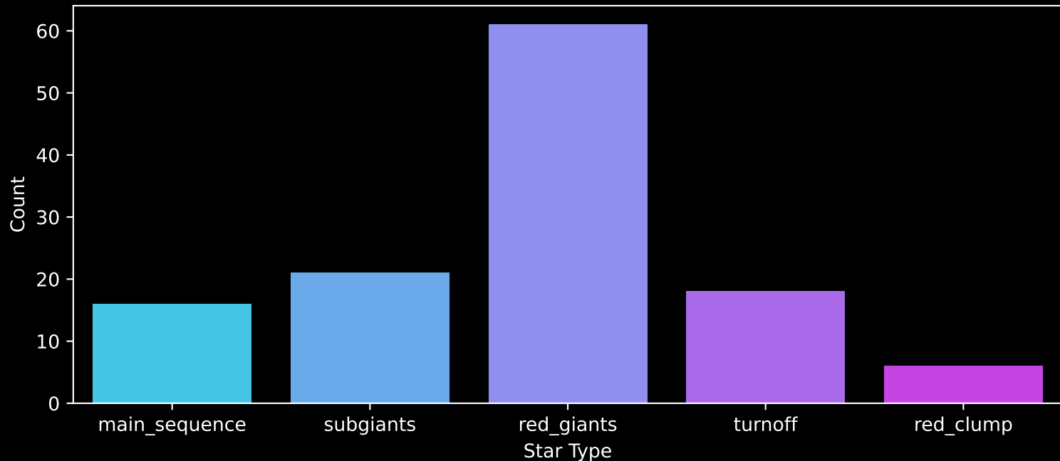
APOGEE DR17 Field: [014+00] Count plot of Star Type
