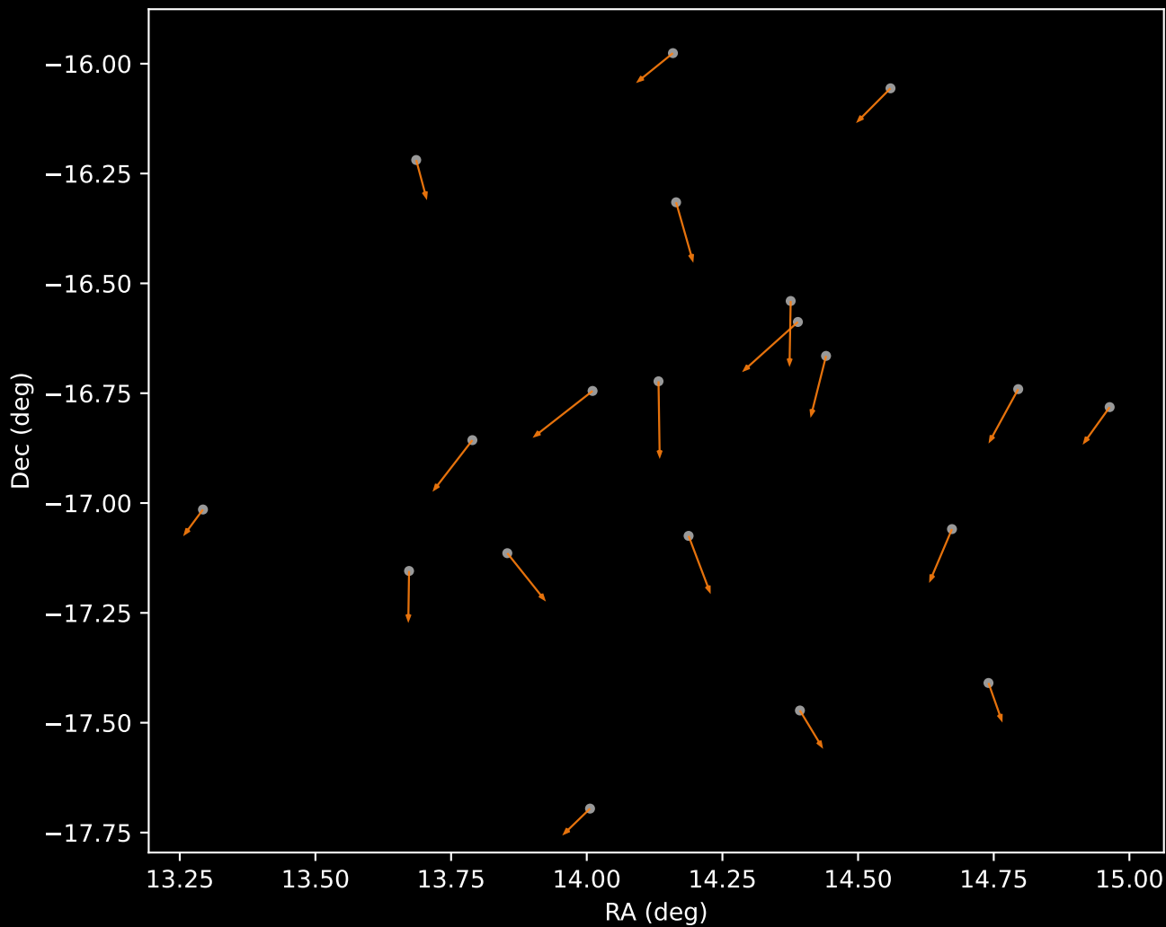
APOGEE DR17 Cluster 2 Proper Motion Vectors (n=20)
