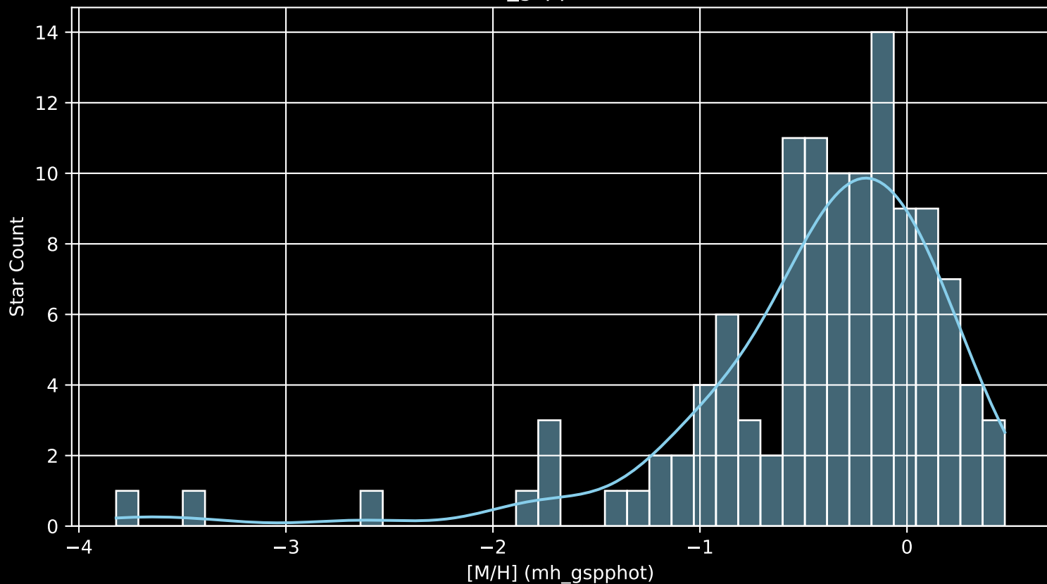
APOGEE DR17 Field: [014+00 [M/H] (mh_gspphot) (n= 116)
